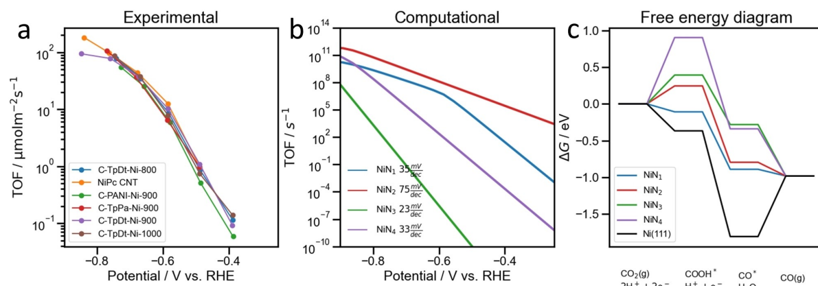
Figure 4. a) The experimentally derived CO turnover frequency (TOF) from -0.4 to -0.85 V RHE , normalized by Ni–N x site density (SD). Apparent Tafel slopes are approximately 100 mV dec. -1 b) Theoretical TOF obtained from a micro-kinetic model of the CO 2 (g) to CO(g) electro-reduction process (calculation detailed in Supporting Information). c) The free energy diagram of CO 2 RR from CO 2 (g) to CO(g) on various DV–Ni–N x ( x = 1, 2, 3, 4 ) motifs and Ni(111) facet at -0.8 V SHE in pH 4. The projected density of state (PDOS) plots of all studied Ni–N x motifs are displayed in Figure S16.
